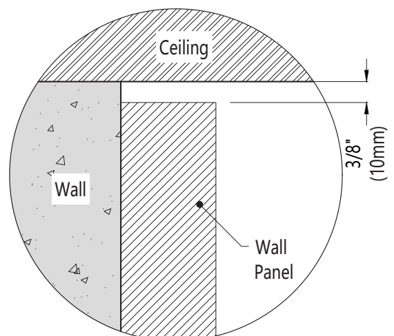
Detail 3-4
