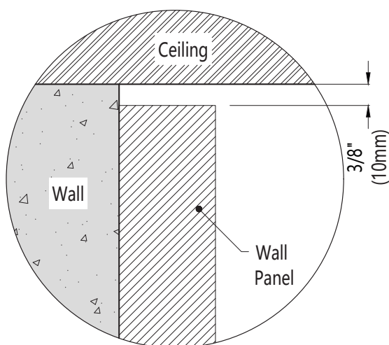
Detail 3-1
