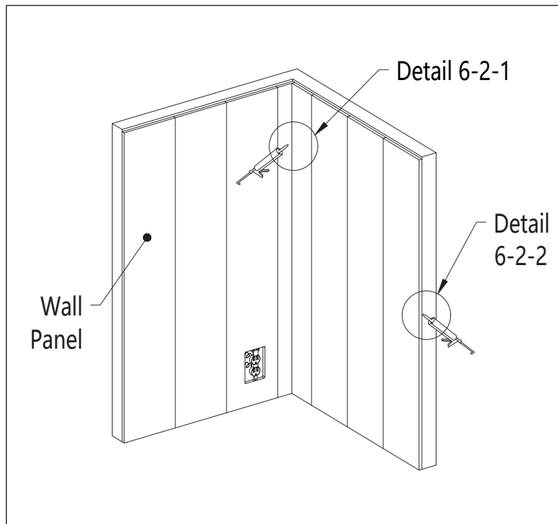
Diagram 6-2
